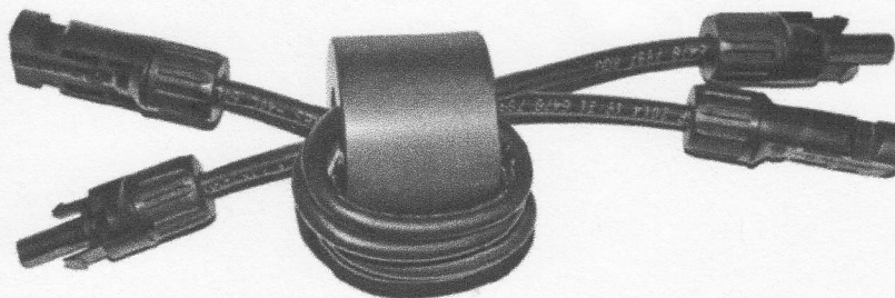
Figure 5 — Three bifilar turns of #10 PV wire on Fair-Rite 2631626202 core with MC4 connectors installed.
