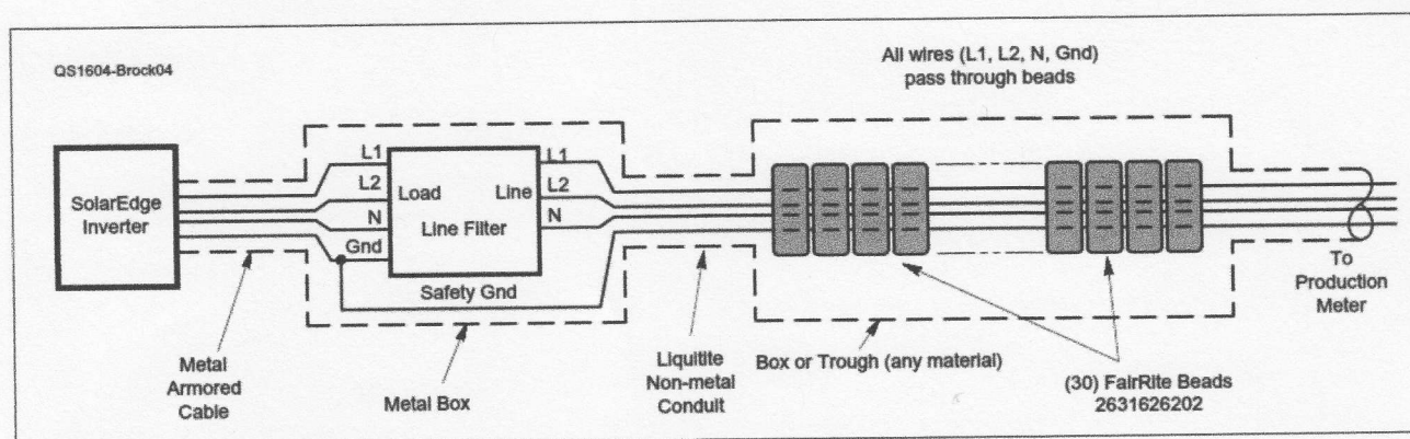
Figure 4 — Line filtering of ac between the inverter and line connection.
