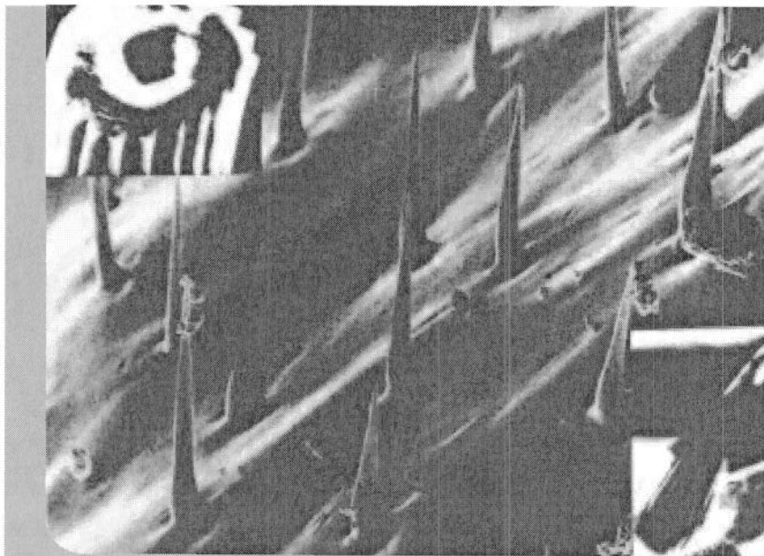
Fig. 15: Wing section of bees enlarged with scanning electron microscope. Observe the special structures serving to focus the electrical field. Warnke 1989, Copyright Ulrich Warnke
