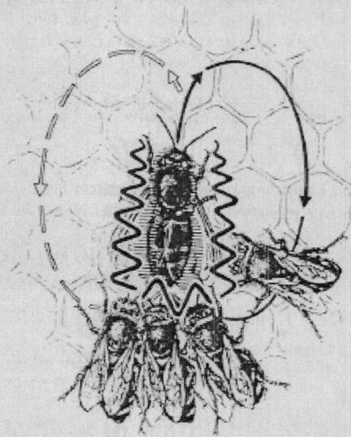
Fig. 21: The waggle dance of the bees generates electrical oscillating fields. Warnke 1989, Copyright Ulrich Warnke
