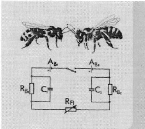
Fig. 3: Bees communicate via electrical "switching" when their antennae touch. Warnke 1989, Copyright Ulrich Warnke
