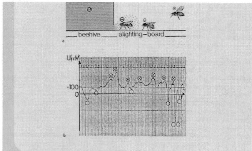
Fig. 10: Every bee landing at the hive carries a specific charge (circle with cross) thereby changing its pattern of charge at the hive entrance, determined by the total electrical charge of the colony. Every departing bee carries with it electrical charge from the hive (circle). Warnke 1989, Copyright Ulrich Warnke
