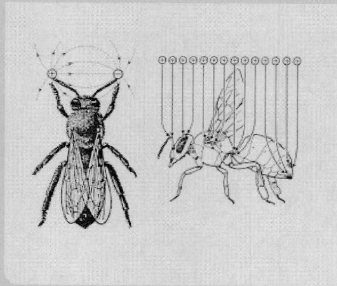
Fig. 14.1: Representation of a measurable "dipole effect" on the antennae of the honeybee. Bees are able to change the polarity of their antennae at will (e.g. from positive to negative charge) – within a second. The dotted lines are an indication of the forces in the field.
