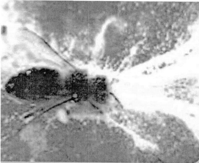
Fig. 12: Bee in flight in an electric field. The fields around the antennae are particularly strong.
